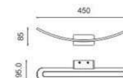
W17608-10W POWER : 10W SIZE(mm) : L450×W85×H95 COLOUR : WHITE
