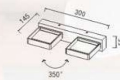
W17606-10W POWER : 10W SIZE(mm) : L300×W145×H55 COLOUR : WHITE
